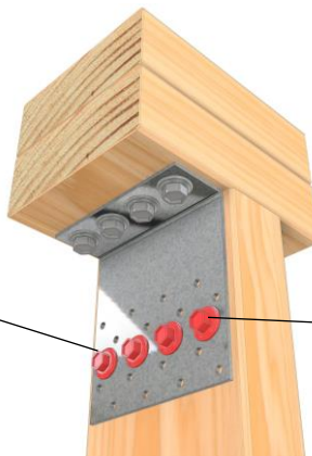
4 x Pryda 12G x 35mm Timber Connector screws.
