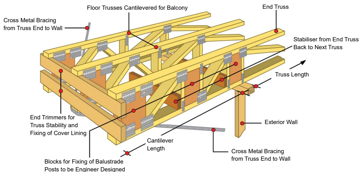
Figure 34: Cantilevered truss end detail.
