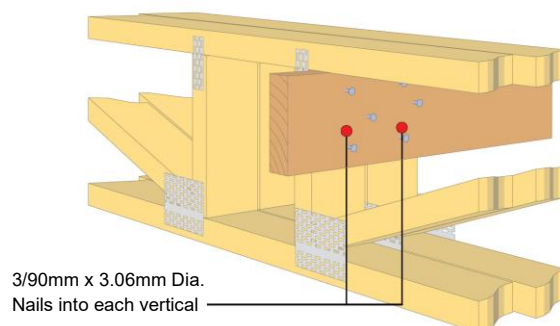
Figure 33: Multiple truss fixing.
