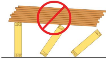
Figure 16: Don't stack materials on unbraced trusses.
