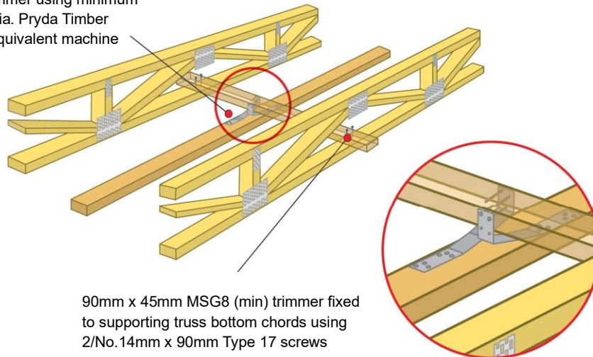
Figure 25: Walls parallel.
