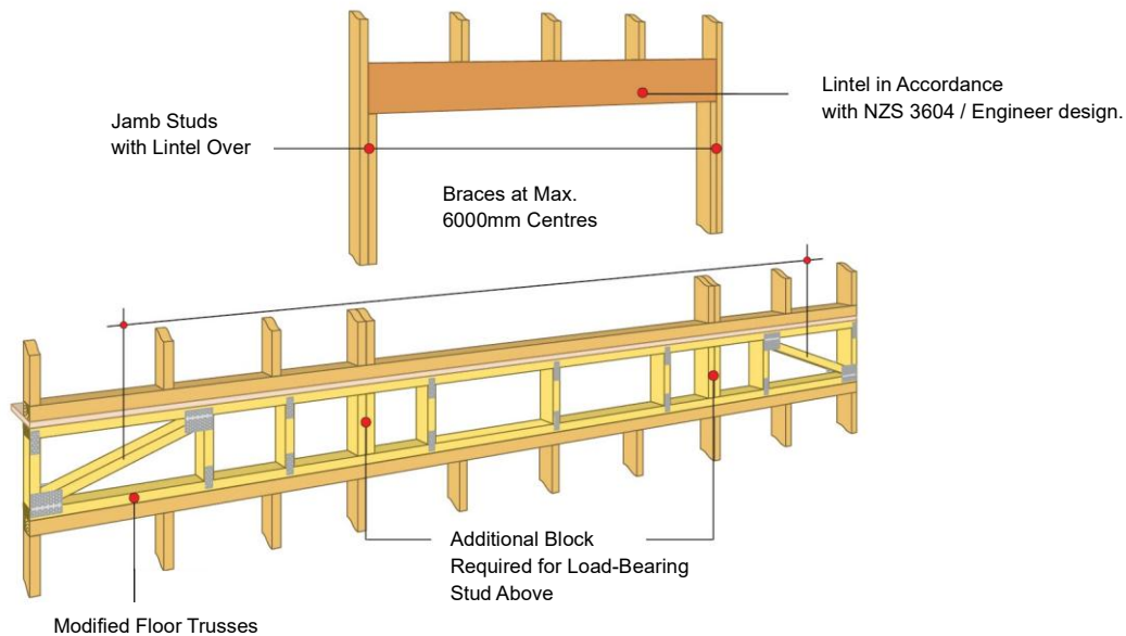
Figure 29: Fully supported end truss.
