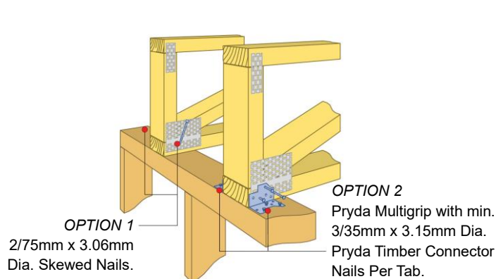
Figure 9: Typical plate support fixing.
