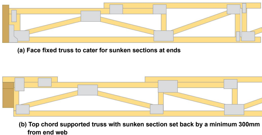
Figure 24: Sunken Sections support types.
