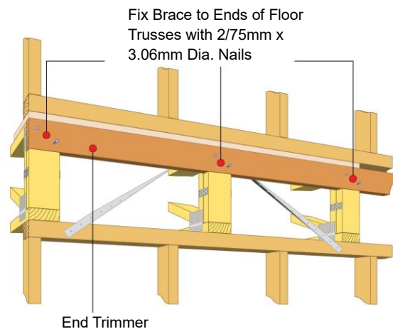
Figure 6b: Brace not wrapped under the wall plate is not recommended.
