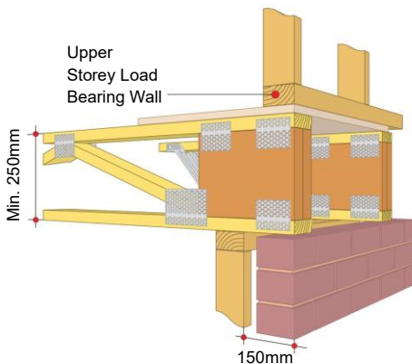
CANTILEVER - PARALLEL OFF-SET UPPER LOAD BEARING WALL
