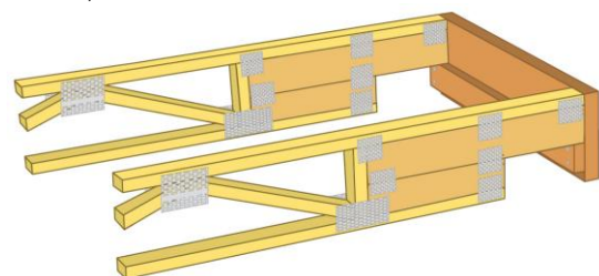
END DETAIL TYPE 5.4 (Pelmets or box gutter when used as rafter truss)
