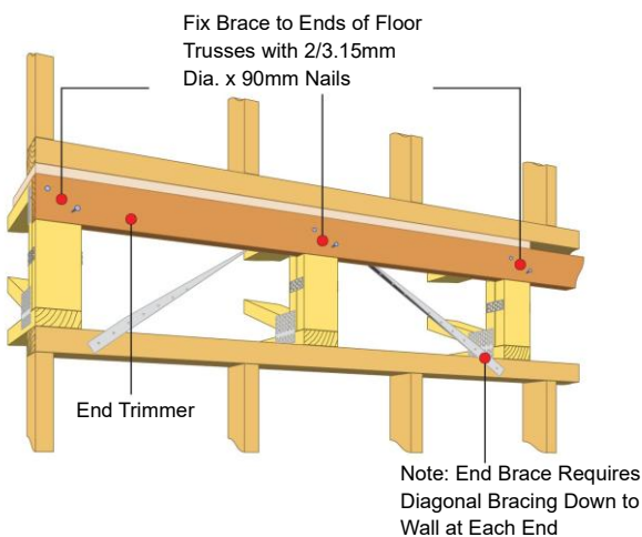
END BRACING FOR STABILITY
