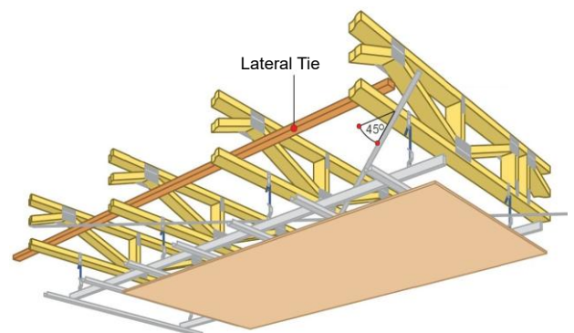
Dynamics of different beam types, floor truss spans and loading conditions shall be assessed simultaneously as a system.
