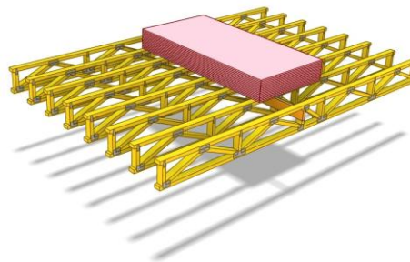
Stacking of material perpendicular to trusses
