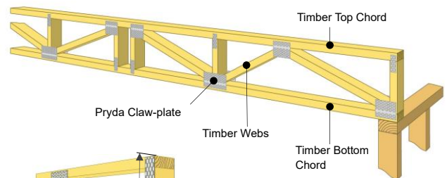
PRYDA LONGREACH TRUSS
