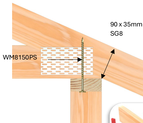
Truss standard heel to top plate
